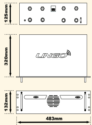
Dimensions (3u form factor)
